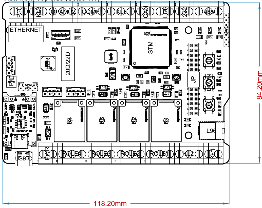
View from Top side (Scale 1:1)
